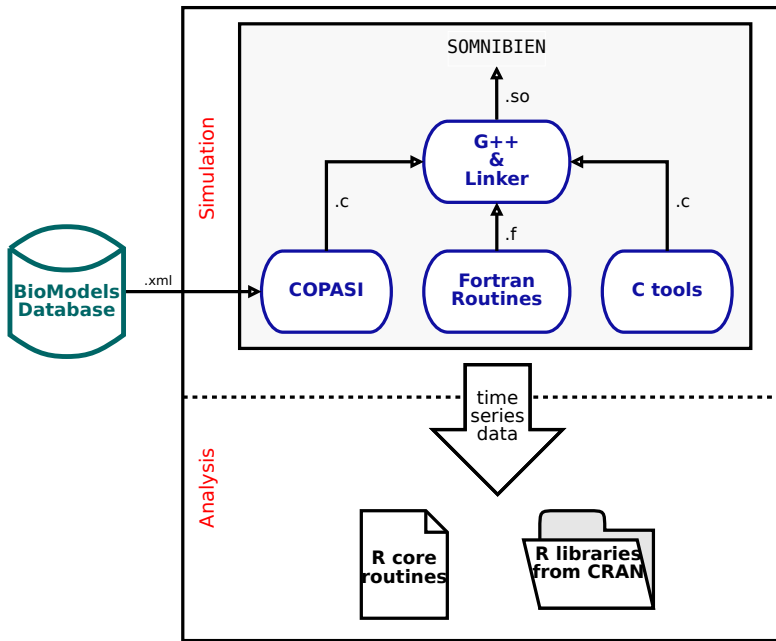
Figure 2: Basic workflow of our system. Models are downloaded as XML-files from the Internet or loaded from the file system. Various calls to external components (COPASI, g++ compiler, linker) compile SBML to C, combine this with numerical code in Fortran, and tool infrastructure in C into an object file, that can be called from within SOMNIBIEN and therefor R. This enables the user to analyze the simulated data directly within R using its superb analysis procedures as well as additional R-software from repositories such as CRAN [cra].
