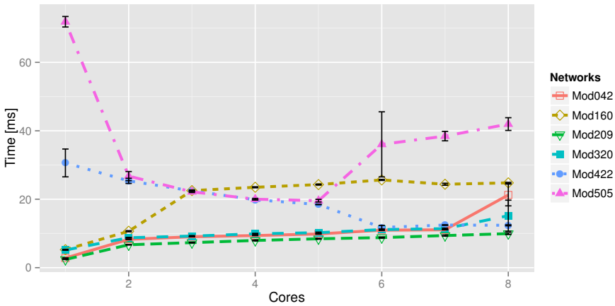
Figure 5: Execution times of an integration step averaged over the six different metabolic networks of Tab. 1 without internal noise ( \beta = 0 in Eq. 4). Each network was simulated 100 times on the given number of cores. Error bars show the standard deviation.
